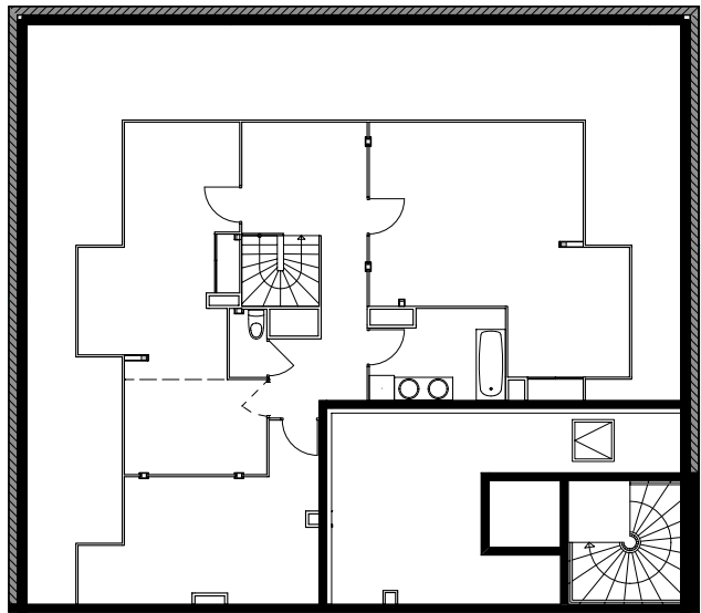
PLANS COMBLES
